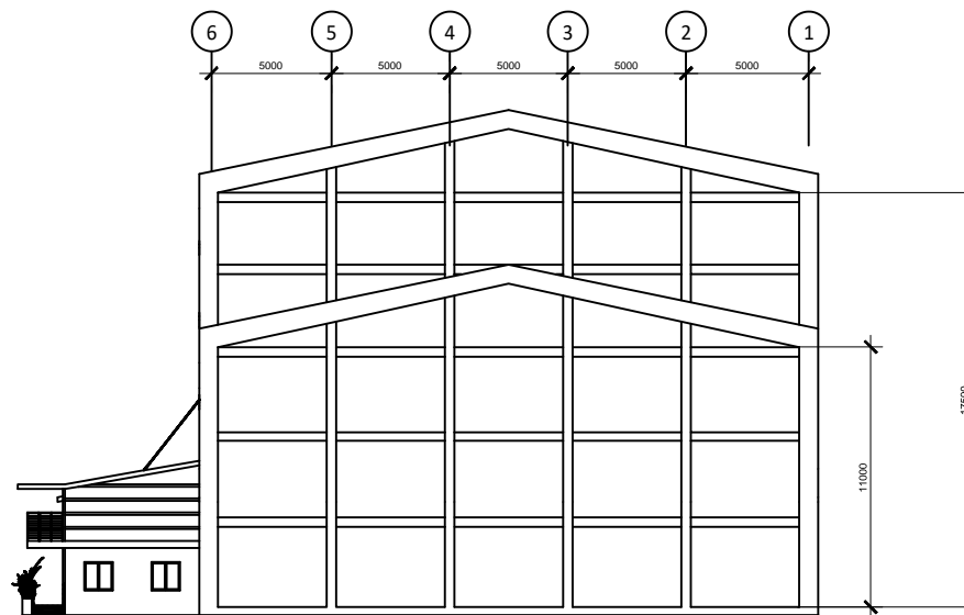
REAR VIEW
